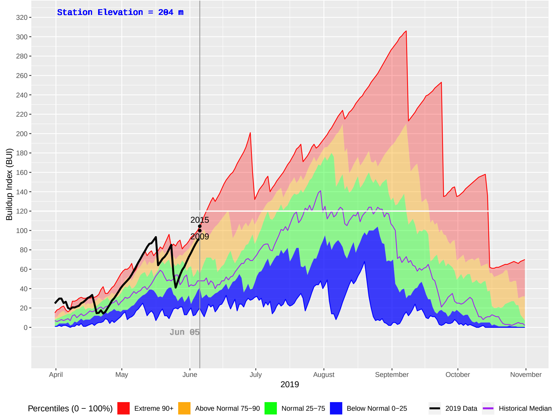
PEMBERTON BASE (301) : Historical (2001–2018), Current (2019) Daily Buildup Index (BUI)
