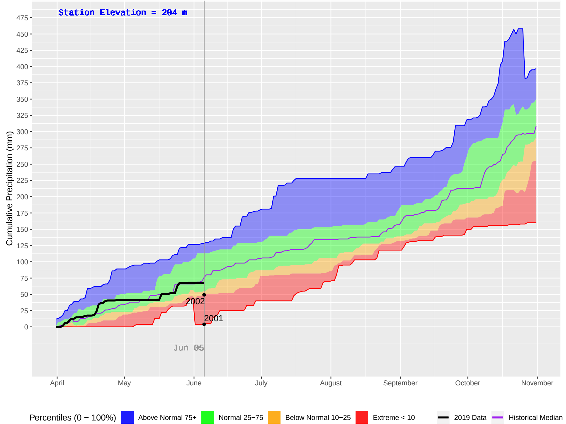
PEMBERTON BASE (301) : Historical (2001–2018), Current (2019) Daily Cumulative Precipitation
